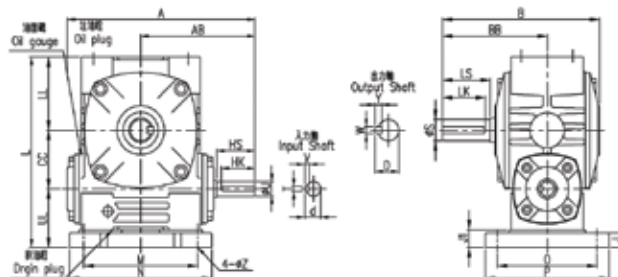
軸配置 SHAFT DIRECTION
